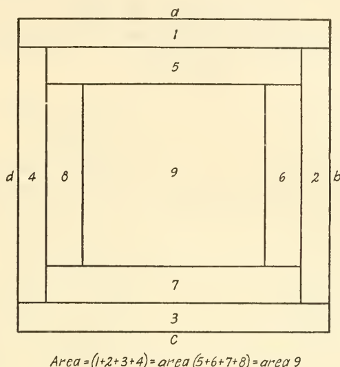
FIGURE 7.—Standard position diagram for moisture-distribution determinations
